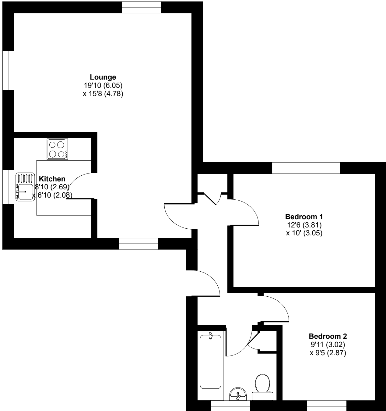
FIRST FLOOR
